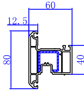
60 Outward Window Sash 310300
