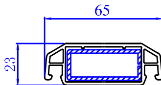
88 Mosquito Sash Mullion 321700
