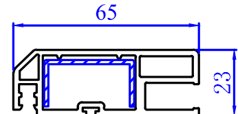
88 Mosquito Sash 321900
