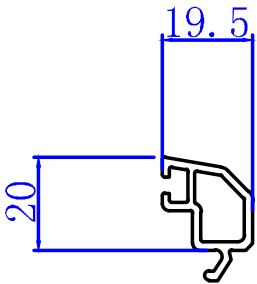
Glazing Bead 19.5 320100
