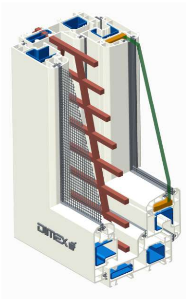
Villa Window Mosquito Sash 330020
