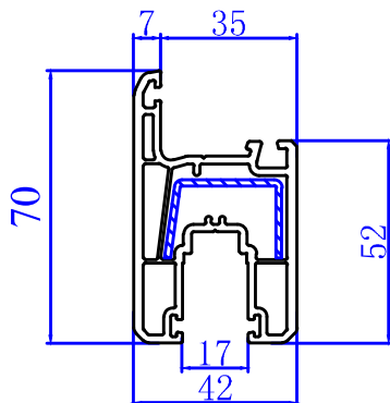
88 Sliding Sash 311000
