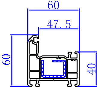
60 Window Frame 310100
