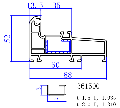
88 Mosquito Sash 321900
