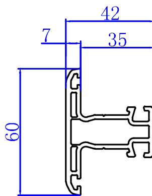
88 Mosquito Sash Mullion 321700
