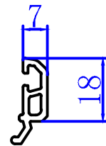
Glazing Bead 7 320300
