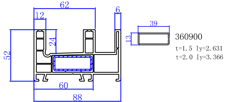
88 Sliding Mullion 311700
