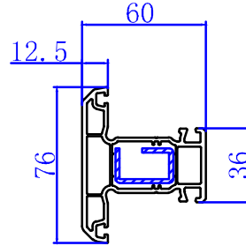
60 Window Mullion 310400
