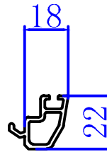
Glazing Bead 22 321200
